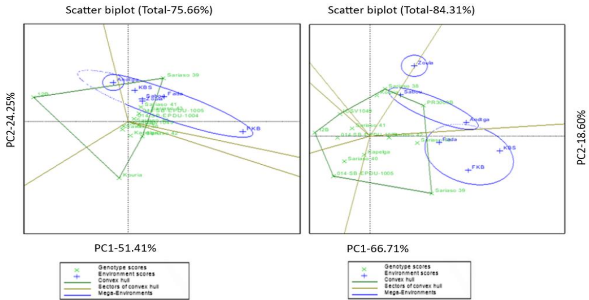
Fig. 1a. Polygon view of the GGE biplot showing mega-environment based on heading time
