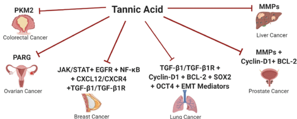
Fig. 3. Showing the Molecular Mechanism of Tannin [46]
