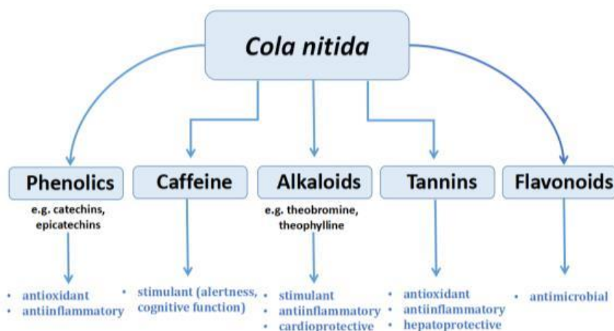
Fig. 2. Showing bioactive ingredients of Cola nitida [25]
