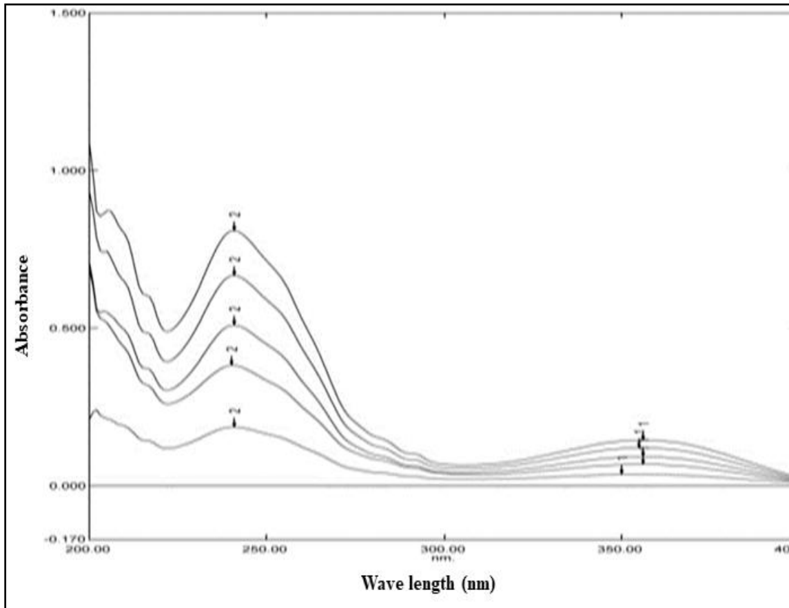
Fig. 2. UV overlay spectrum of Cilnidipine
