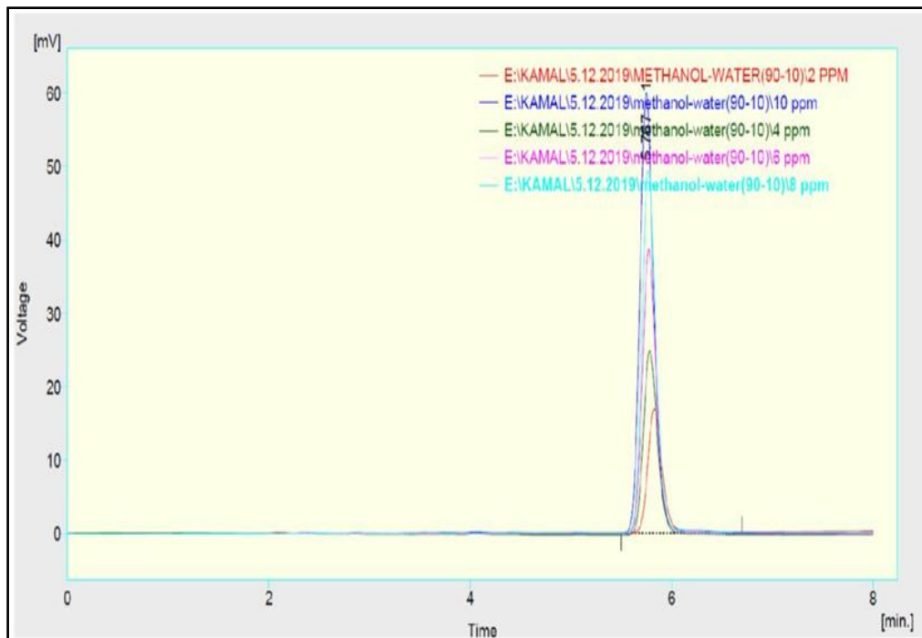
Fig. 3. RP-HPLC overlay spectrum of Cilnidipine
