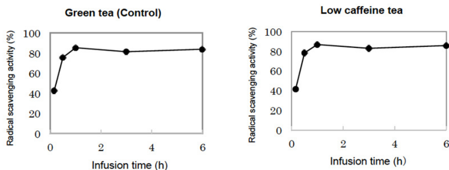
Fig. 2. Comparison of anti-oxidative activity in green tea and low caffeine tea
