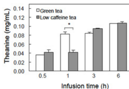
Fig. 1. Quantitative determination of the main components in low caffeine tea
